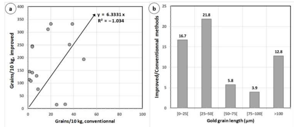
Figure 11. (a) Comparison of the conventional and improved methods in gold grain counts per sample for 15 paired samples. (b) Comparison of the ratio of the number of grains per 10 kg for the improved versus the conventional methods, according to grain size brackets.
