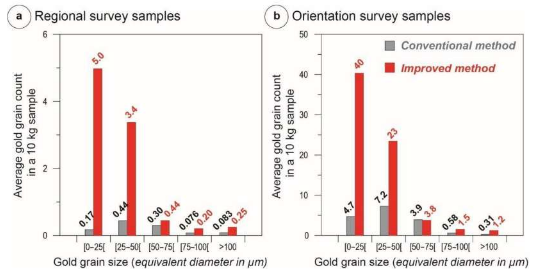
Figure 10. Comparison of the size distribution of the average gold grain count in a 10 kg (–1 mm) sample for the conventional and improved methods. Gold grain size distribution of (a) regional till samples and (b) orientation till samples collected around the Borden gold deposit. See the text for further details. It should be noted that the vertical scale for the orientation samples (b) is 8.3 \times the vertical scale of the regional samples (a).
